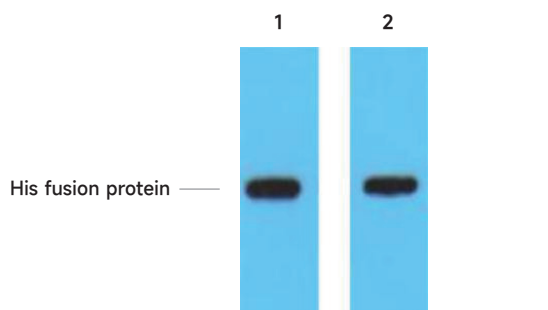
His-Tag 兔多克隆抗体检测 1 \mu g His 融合蛋白 Western Blot 结果【1:5,000(1)、1:10,000(2)】
