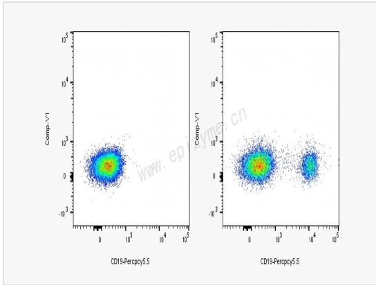
Typical flow-cytometry plots of human peripheral-blood leukocytes stained with anti-CD19-PerCP-Cy5.5 (F100611) (right) compared to unstained control (left).
