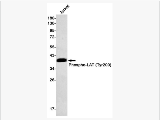
Western blot analysis of Phospho-LAT (Tyr200) in Jurkat lysates using Phospho-LAT (Tyr200) antibody [96L72M05].
