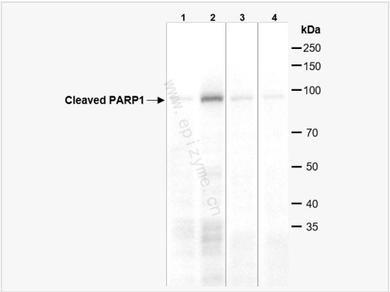
Western Blot - Anti-Cleaved-PARP1 Rabbit mAb [11L11K72] All lanes: R012387 at 1:1,000 dilution Lane 1: HeLa (Human cervix adenocarcinoma epithelial cell) whole cell lysates Lane 2: Jurkat (Human T lymphocytic leukemia cell) whole cell lysates Lane 3: SW620 (Human colorectal carcinoma epithelial cell) whole cell lysates Lane 4: HepG2 (Human hepatocellular carcinoma epithelial cell) whole cell lysates Lysates/proteins at 10 µg per lane. Secondary antibody: Goat Anti-Rabbit IgG(H+L), HRP Conjugated (Cat. No. LF102) at 1:5,000 dilution Predicted band size: 89 kDa Observed band size: 89 kDa Developed using the ECL technique (Cat. No. SQ201).
