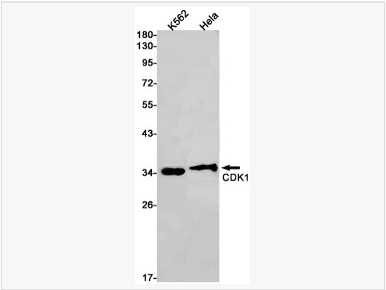
Western blot analysis of CDK1 in K562, HeLa lysates using CDK1 antibody.
