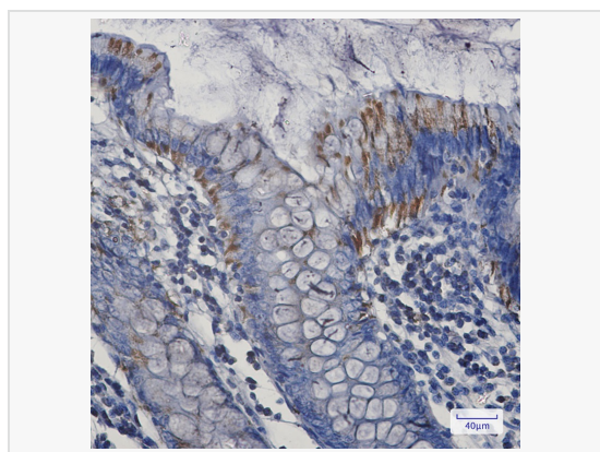
Immunohistochemistry analysis of paraffin-embedded Human colon cancer using Bak antibody. High-pressure and temperature Sodium Citrate pH 6.0 was used for antigen retrieval.
