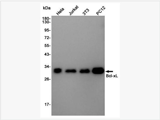
Western blot analysis of Bcl-XL in HeLa, Jurkat, 3T3, PC-12 lysates using Bcl-XL antibody.
