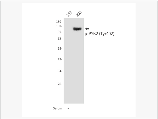
Western blot analysis of Phospho-PYK2 (Tyr402) in 293 lysates using Phospho-PYK2 (Tyr402) antibody.
