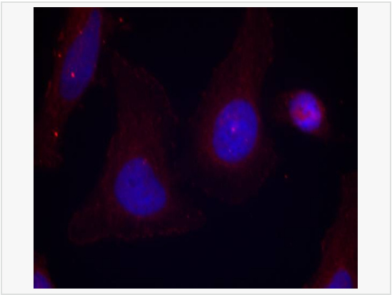
Immunofluorescence analysis of Phospho-PYK2 (Tyr402) in Hela cells using Pyk2 (Phospho-Tyr402) antibody (red) .
