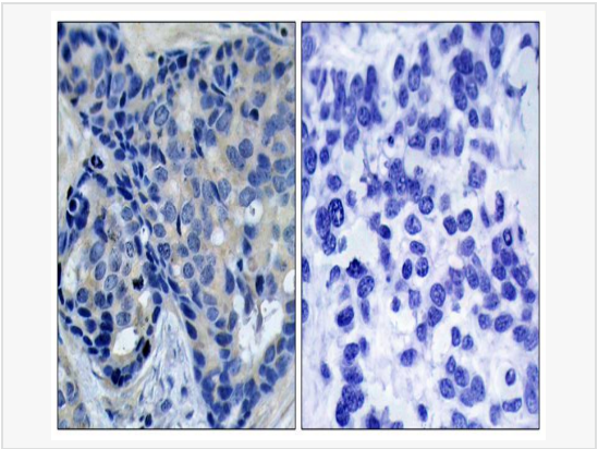
Immunohistochemistry analysis of paraffin-embedded Human breast carcinoma tissue using Pyk2(Phospho-Tyr402) antibody. High-pressure and temperature Sodium Citrate pH 6.0 was used for antigen retrieval. Sample with blocking peptide on the right.
