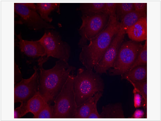
Immunofluorescence analysis of Phospho-Estrogen Receptor alpha (Ser167) in MCF-7 cells using Estrogen Receptor alpha (Phospho-Ser167) antibody (red) .
