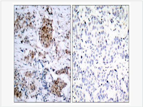
Immunohistochemistry analysis of paraffin-embedded Human breast carcinoma tissue using Estrogen Receptor alpha (Phospho-Ser167) antibody. High-pressure and temperature Sodium Citrate pH 6.0 was used for antigen retrieval. Sample with blocking peptide on the right.
