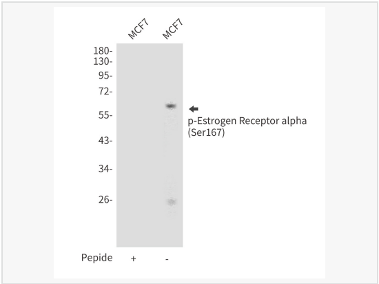
Western blot analysis of Phospho-Estrogen Receptor alpha (Ser167) in MCF-7 lysates using Phospho-Estrogen Receptor alpha (Ser167) antibody.
