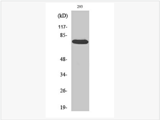
Western blot analysis of Raf1 in various lysates using Raf1 antibody.
